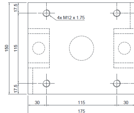
Upper plate
